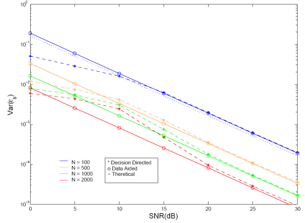
Fig. 4. Estimation error for 16 QAM constellation and different values of N .
