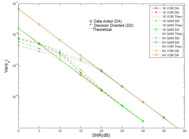
Fig. 5. Estimation error comparison between different constellations with N=1000 .
