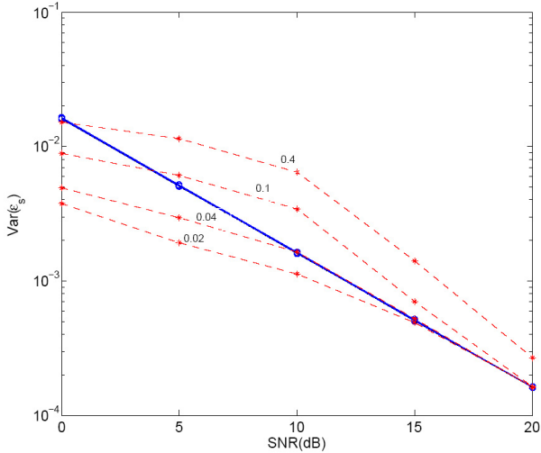
Fig. 2. Estimation error for the data-aided estimator (solid line) and the decision-directed (dashed-line) different values of \sigma_g^2 .
