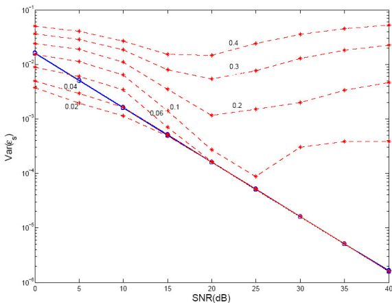
Fig. 3. Behavior of estimation error for 16 QAM constellation with different values of \sigma_g .
