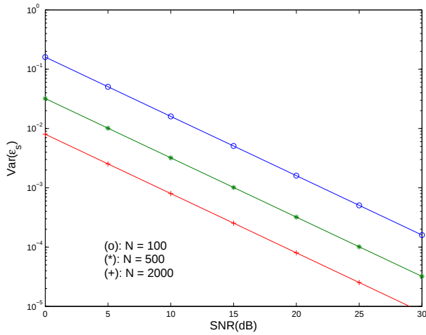
Fig. 1. Estimation error for the data-aided estimator with different values of N (markers denote simulated values).
