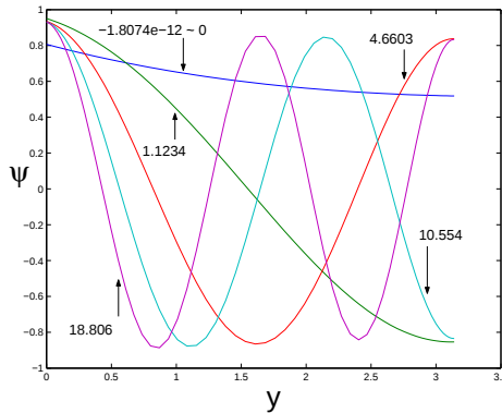
Figure 2: Plot of graviton wave functions \psi for l/r_c = 5 and p_B^5 = 0.25 . Shown are the massless graviton and the first four massive gravitons. The mass scale is set by r_c = 100\mu m = 1 \times 10^3 \text{eV}^{-1} .
