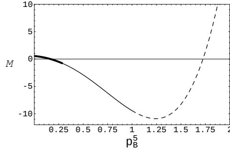
Figure 1: Plot of radion mass parameter M for l/r_c = 5 . Thick line, 0 < p_B^5 \leq e^{-2\pi/5} : \lambda > 0, \lambda' \leq 0 . Thin line, e^{-2\pi/5} < p_B^5 \leq 1 : \lambda \geq 0, \lambda' > 0 . Dashed line, p_B^5 > 1 : \lambda < 0, \lambda' > 0 .
