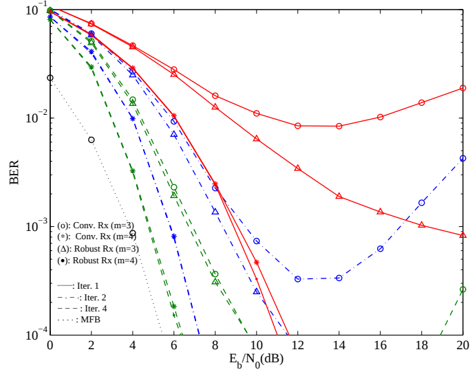
Fig. 12. BER performance for a BS cooperation scenario with P = 2 MTs and R = 2 BSs. Comparison of results with quantization with m = 3 and 4 bits of resolution employing a conventional and robust receivers (2nd MT).
