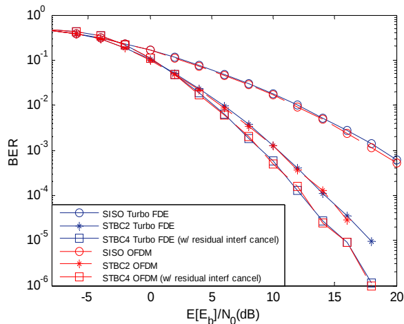
Figure 3. Coded BER for SC-FDE and OFDM.
