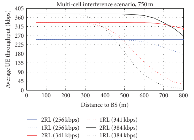
FIGURE 13: Throughput versus distance between UEs and BS, k = 0.5 .
