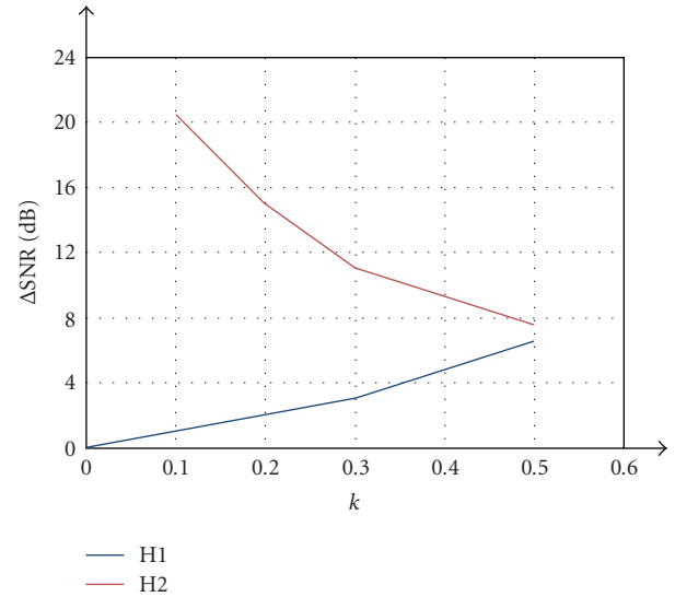
FIGURE 9: ASNR versus k for hierarchical 16-QAM, 256 kbps, VehA 30 km/h.
