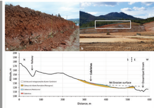
Fig. 3. Top: Profiles: (a) trench; (b) cut made by the construction works. Bottom: Profile made using GPS/RTK showing altitude and stratigraphic units. The profile shows the N4 erosive surface, the colluvium (Pleistocene) and the Cabeço do Infante Formation (Palaeogene).
